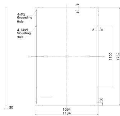
Rear View
